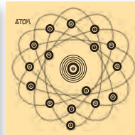
Atom
