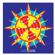
Windrose
